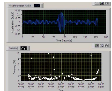
Figure 4: Response and damping reported by the system in February 2007
