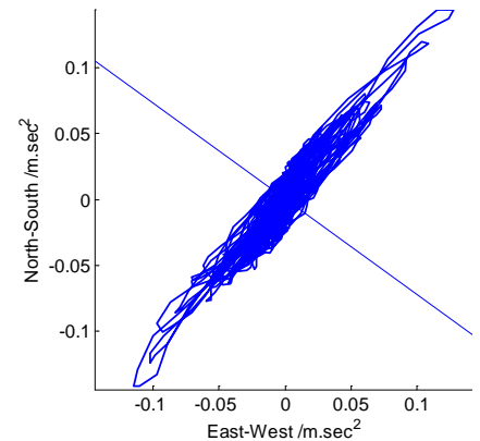
Figure 3: Typical cross-wind response due to vortex shedding
